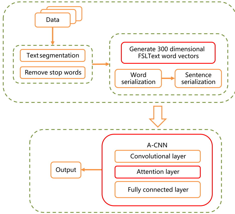
Fig. 1. General architecture of intention detection.
