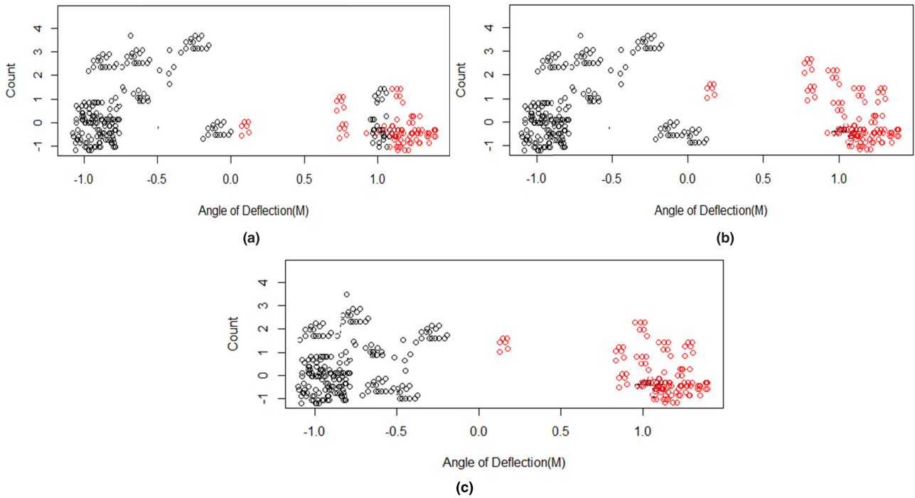
FIGURE 7. Shows clustering results for the two methods IT_KM (b) and EC_G (c) used and compared on the Fish dataset (D3) with K-Means(a). The ensemble clustering method EC_G shows better clustering results in terms of overlapping and inter-cluster distance.
