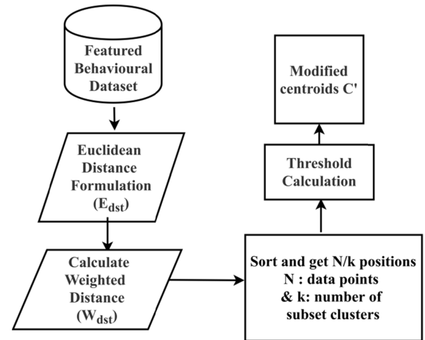
FIGURE 2. IT K M workflow.
