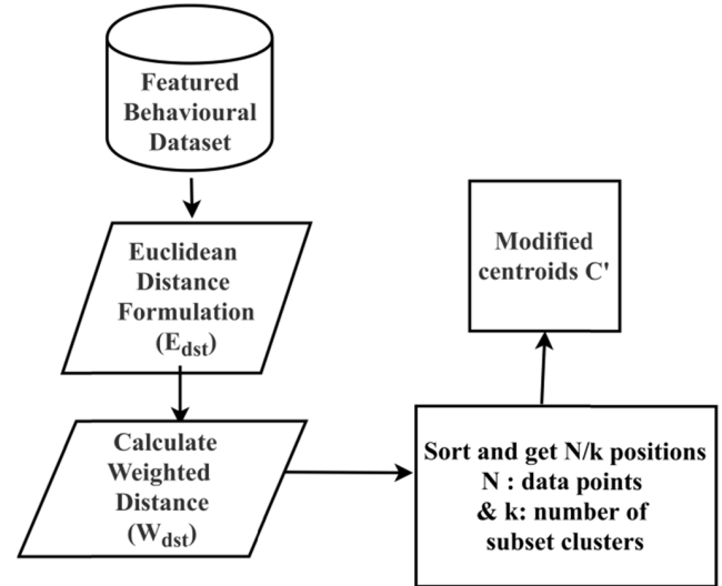
FIGURE 1. IC K M Workflow.
