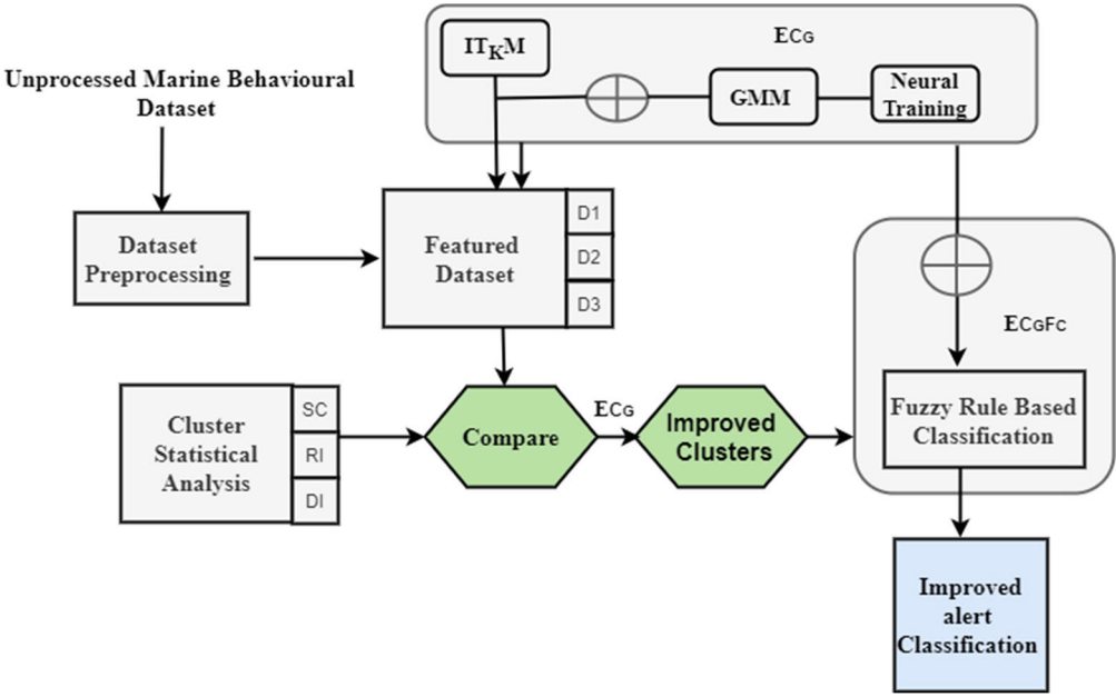
FIGURE 4. The workflow of complete proposed approach: EC G FC.
