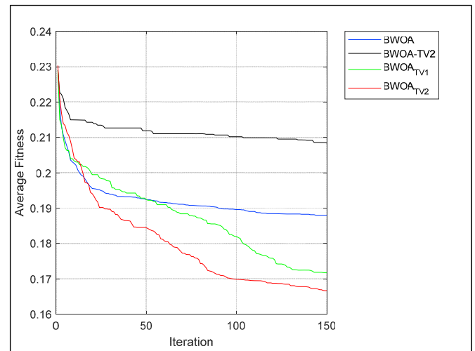
Fig. 3. Convergence curves of proposed BWOA TV1 and BWOA TV2 algorithms with other binary variants of WOA algorithm.
