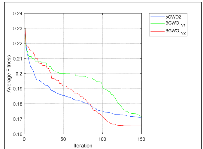
Fig. 4. Convergence curves of proposed BGWO TV1 and BGWO TV2 algorithms with other binary variants of GWO algorithm.
