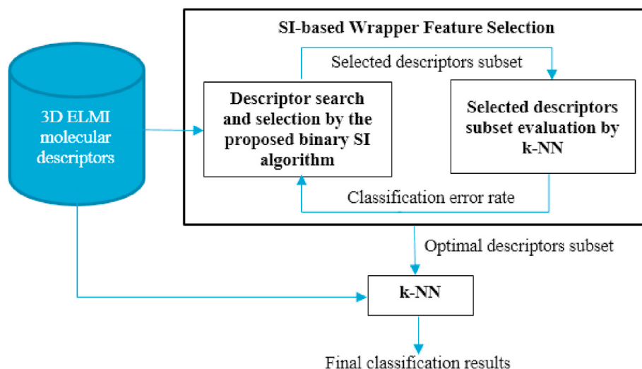
Fig. 1. Framework of the proposed binary SI-based wrapper descriptors selection technique.
