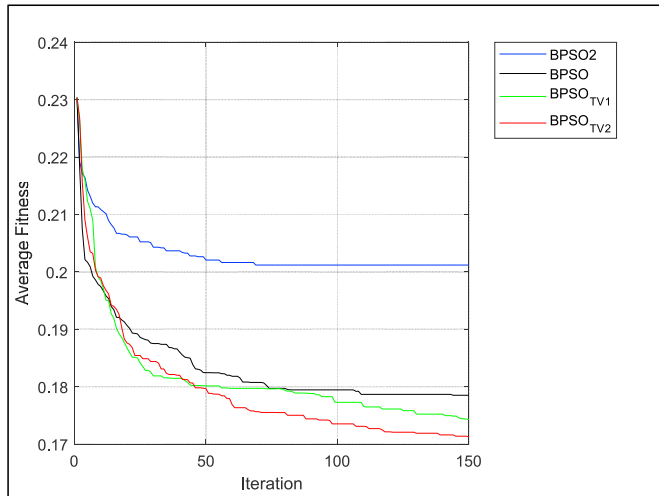
Fig. 2. Convergence curves of proposed BPSO TV1 and BPSO TV2 algorithms with other binary variants of PSO algorithm.
