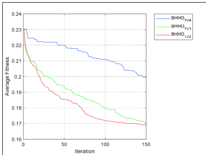
Fig. 5. Convergence curves of proposed BHHO TV1 and BHHO TV2 algorithms with other binary variants of HHO algorithm.
