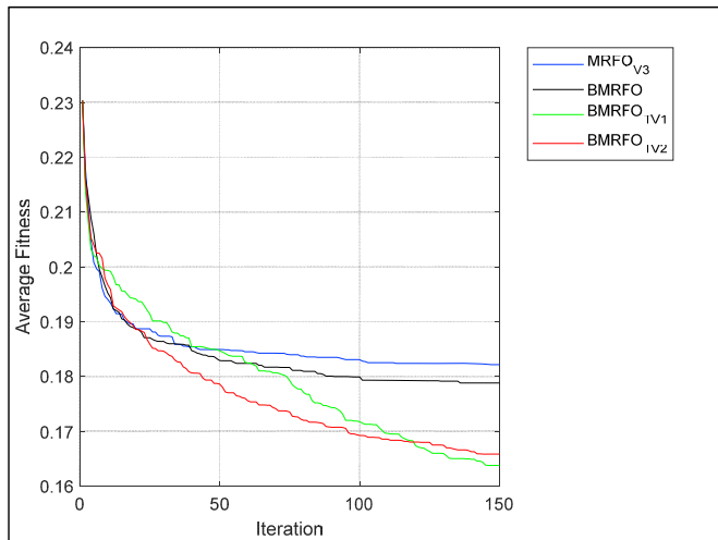
Fig. 6. Convergence curves of proposed BMRFO TV1 and BMRFO TV2 algorithms with other binary variants of MRFO algorithm.
